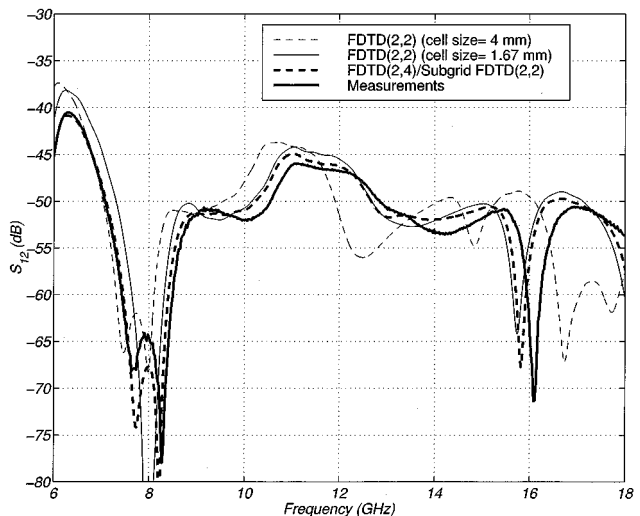
Fig. 3. S_{12} between the two monopoles shown in Fig. 1.
