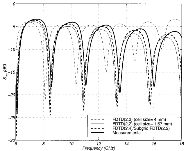
Fig. 2. S_{11} of the 6 cm long monopole shown in Fig. 1.
