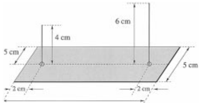
Fig. 1. Geometry of two monopoles on a ground plane.
